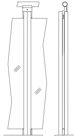
Aztec guardrail post 42" H
