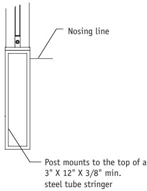
Stair post top mount
