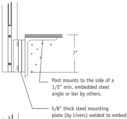
Level post side mount
