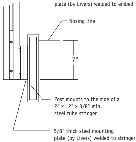
Stair post side mount
