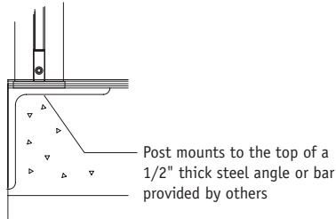
Level post top mount
