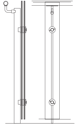
Optional Strata guardrail post 42" H
