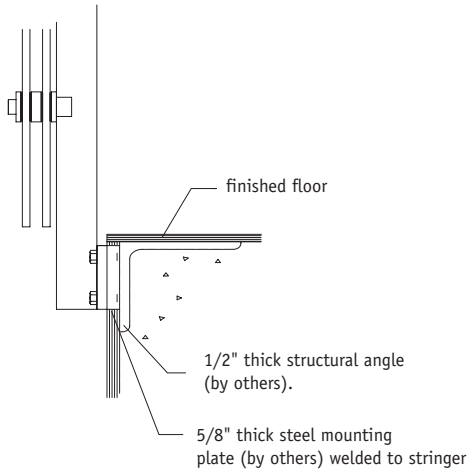
Side mounting detail
