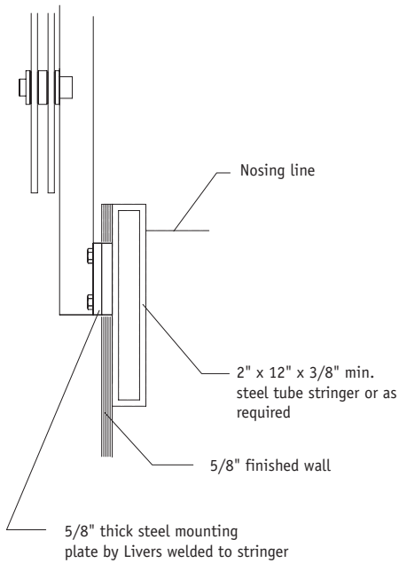
Stringer mounting detail
