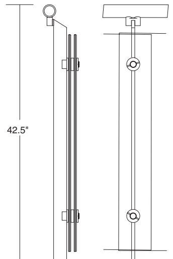
Strata guardrail post 42" H
