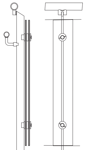
Strata stair rail post 42" H
